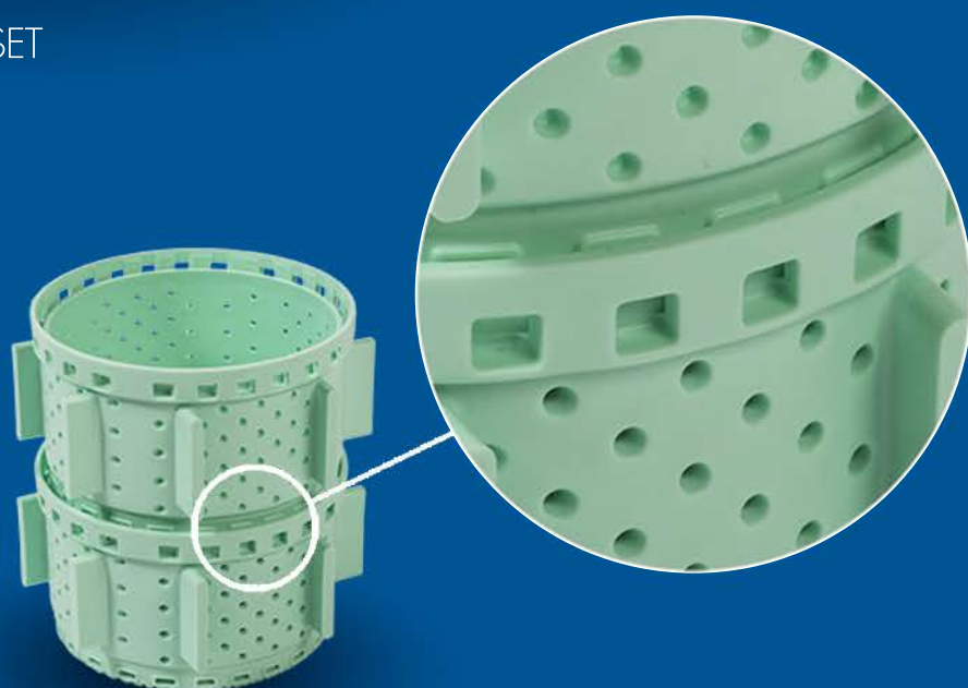
MOULD WITH BOTTOM AND ANTI-DROP SYSTEM
